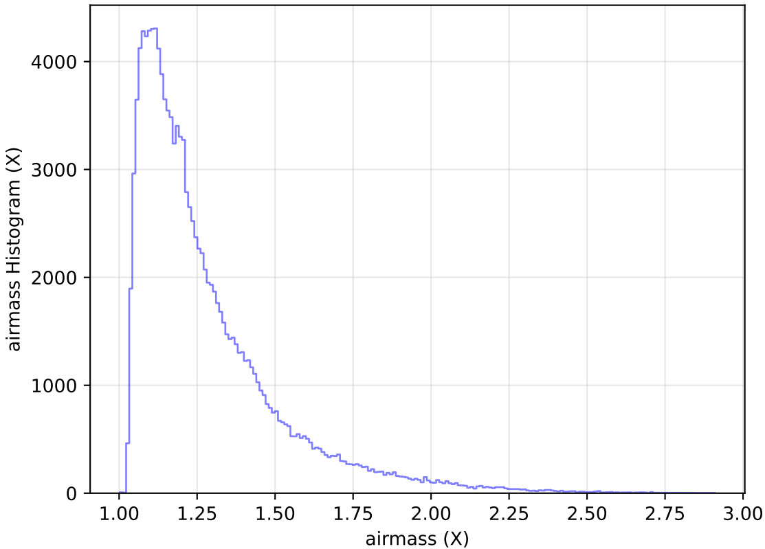
weather_cloudso16v3.4_10yrs WFD u band: airmass Histogram
