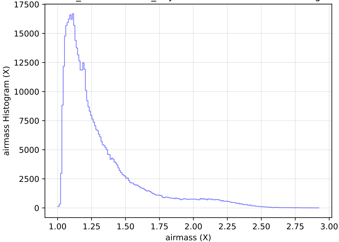
weather_cloudso16v3.4_10yrs WFD r band: airmass Histogram
