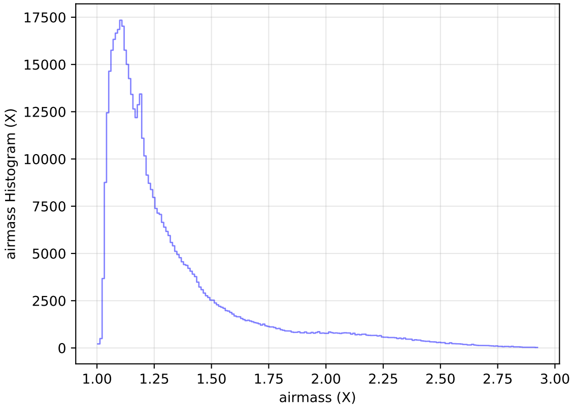
weather_cloudso16v3.4_10yrs WFD i band: airmass Histogram
