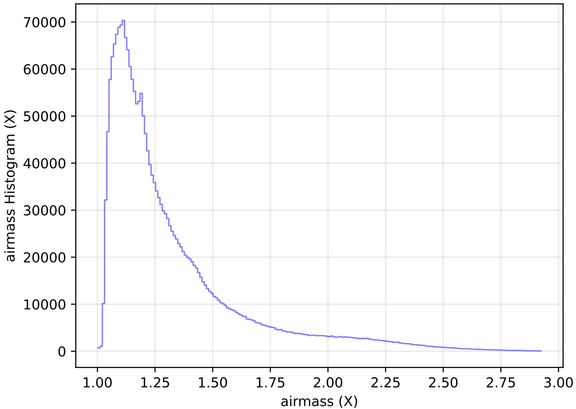
weather_cloudso16v3.4_10yrs WFD all bands: airmass Histogram
