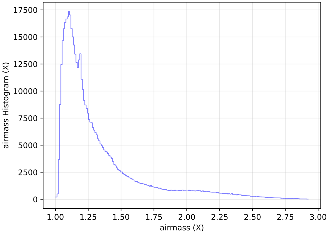
weather_cloudso16v3.4_10yrs All sky i band: airmass Histogram
