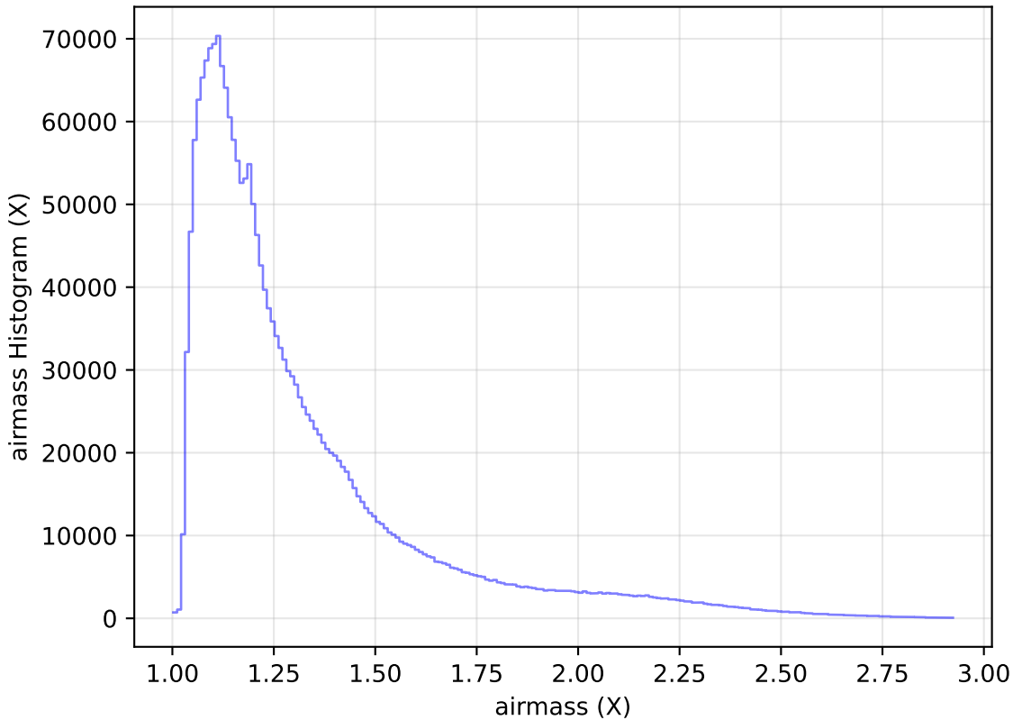
weather_cloudso16v3.4_10yrs All sky all bands: airmass Histogram
