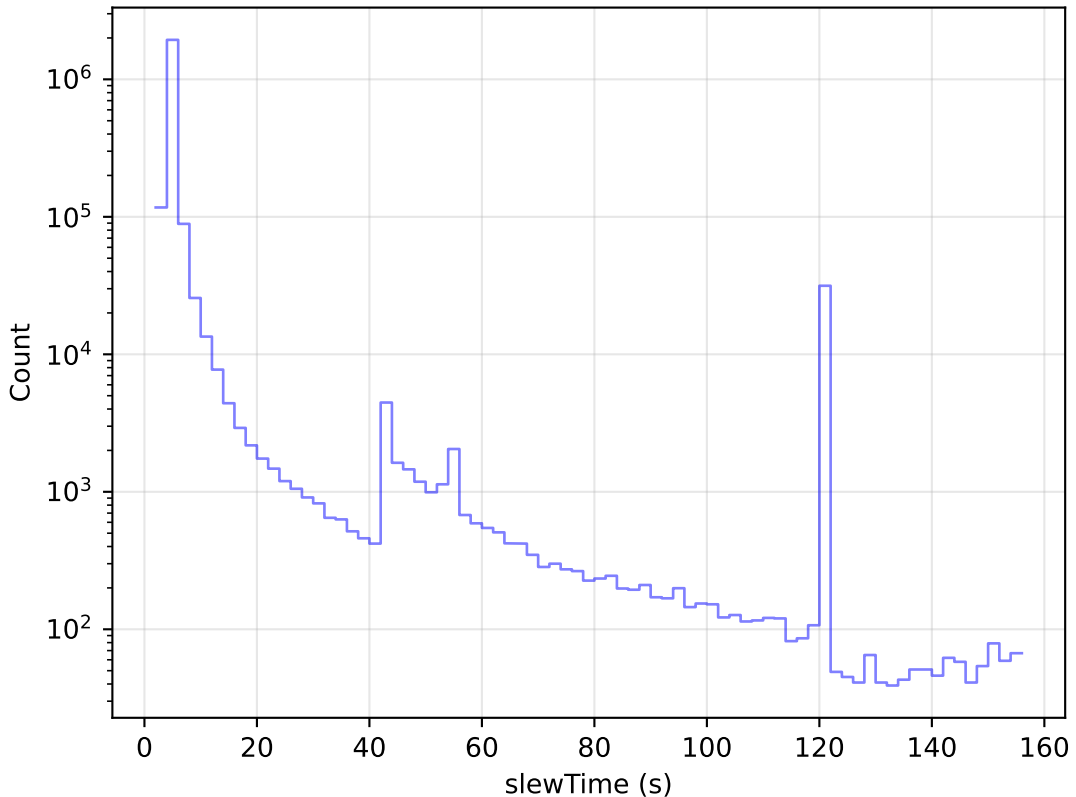
weather_cloudso16v3.4_10yrs All visits: Slew Time Histogram
