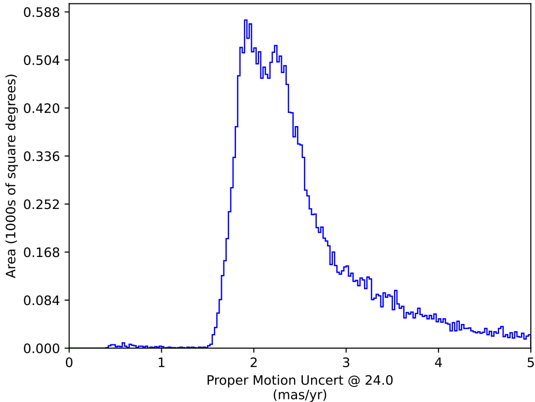
weather_cloudso16v3.4_10yrs All sky: Proper Motion Uncert @ 24.0
