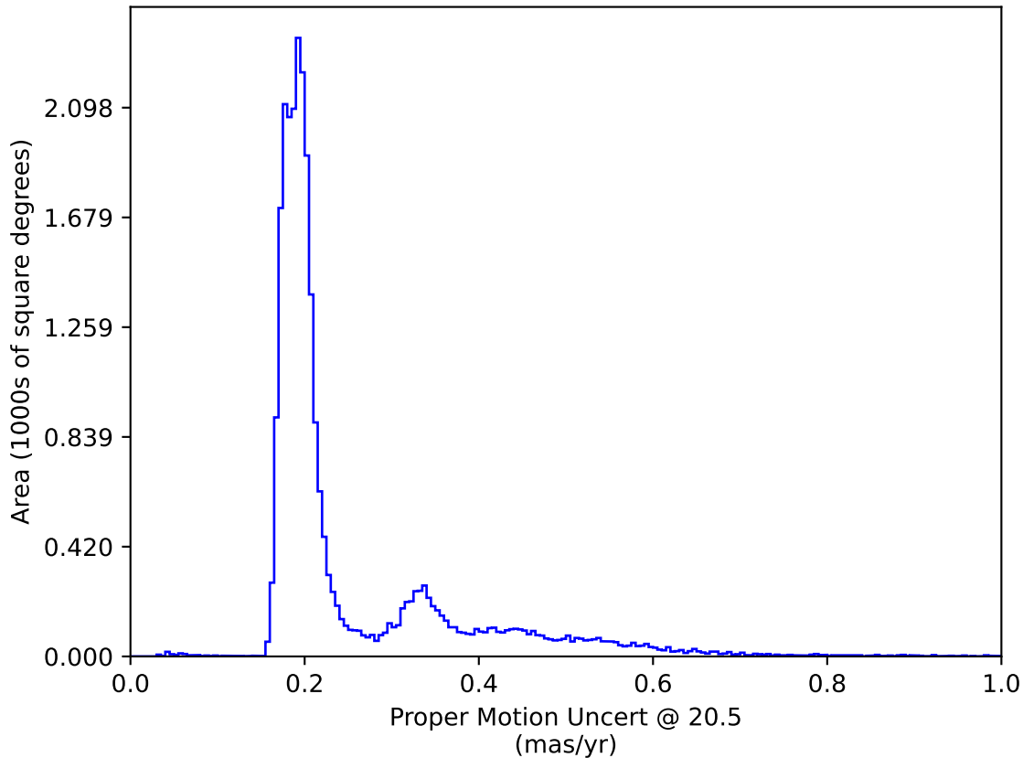
weather_cloudso16v3.4_10yrs All sky: Proper Motion Uncert @ 20.5
