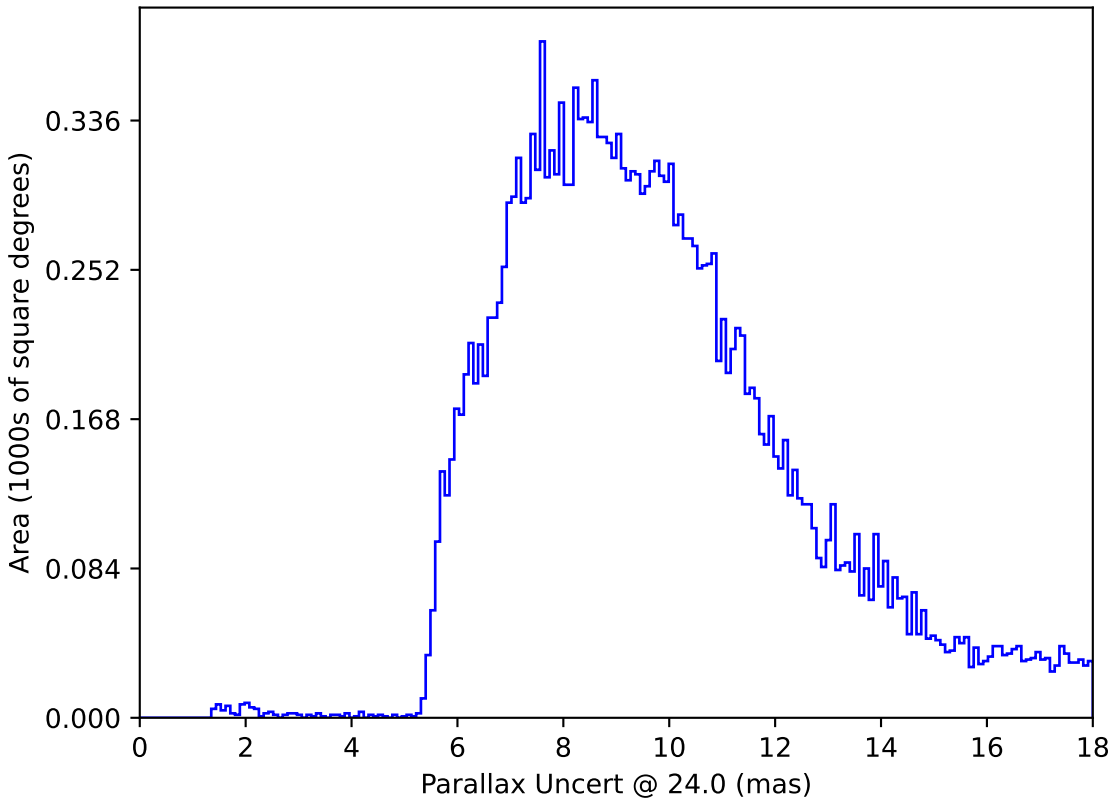
weather_cloudso16v3.4_10yrs All sky: Parallax Uncert @ 24.0
