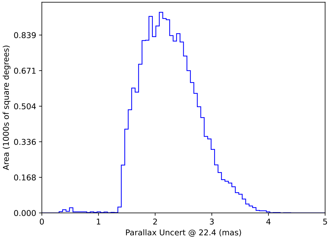
weather_cloudso16v3.4_10yrs WFD: Parallax Uncert @ 22.4
