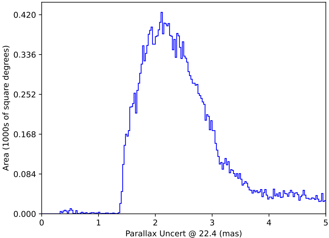
weather_cloudso16v3.4_10yrs All sky: Parallax Uncert @ 22.4
