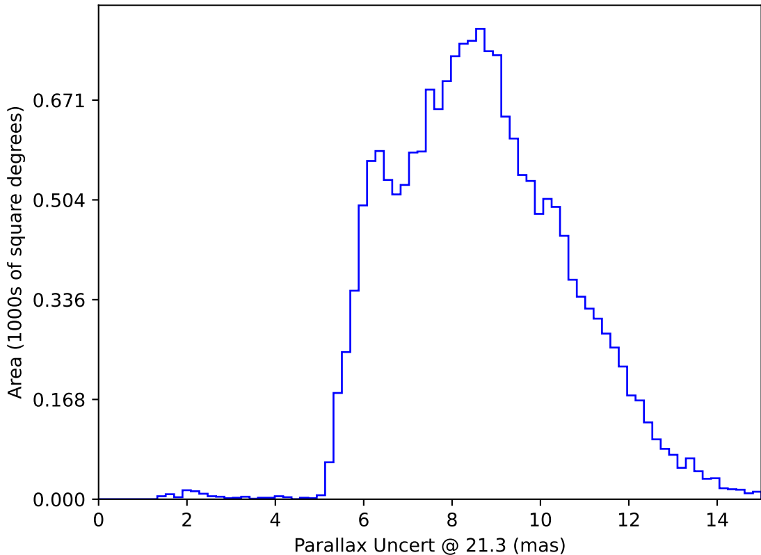
weather_cloudso16v3.4_10yrs WFD y band only: Parallax Uncert @ 21.3
