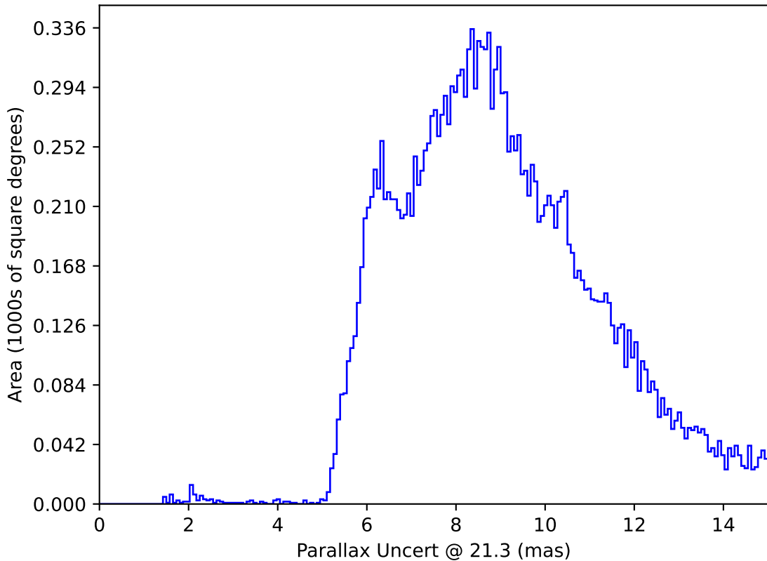
weather_cloudso16v3.4_10yrs All sky y band only: Parallax Uncert @ 21.3
