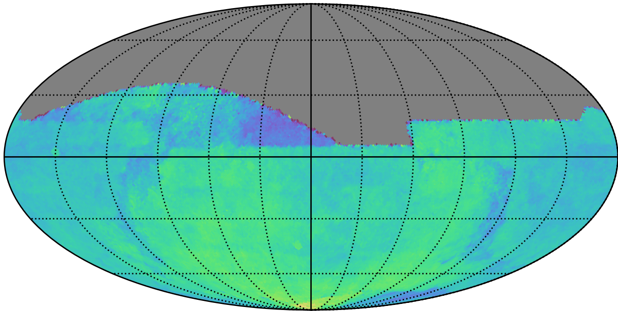
weather_cloudso16v3.4_10yrs All sky: Parallax Coverage @ 24.0
