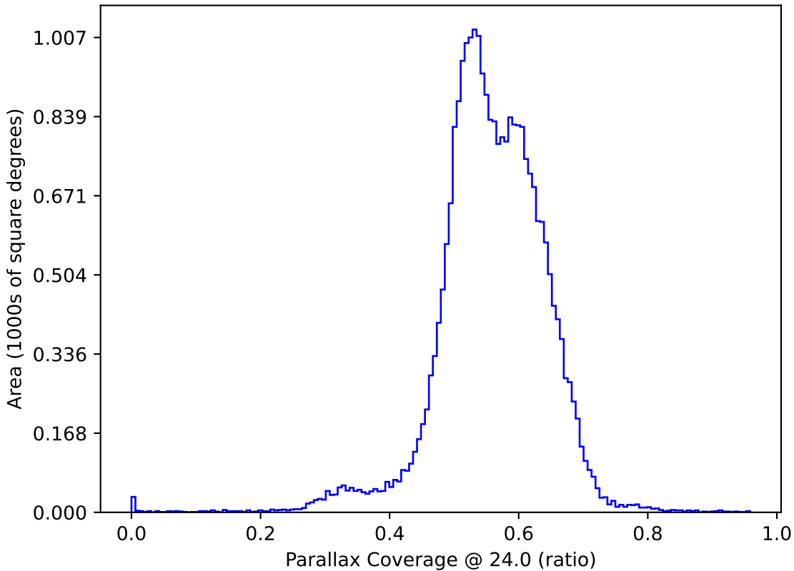
weather_cloudso16v3.4_10yrs All sky: Parallax Coverage @ 24.0
