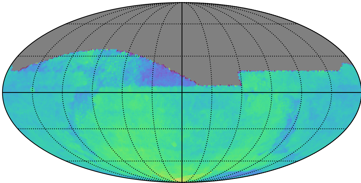
weather_cloudso16v3.4_10yrs All sky: Parallax Coverage @ 22.4
