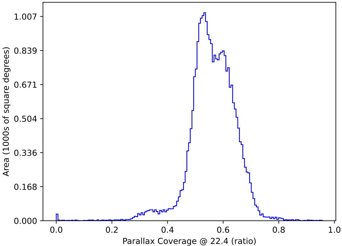
weather_cloudso16v3.4_10yrs All sky: Parallax Coverage @ 22.4
