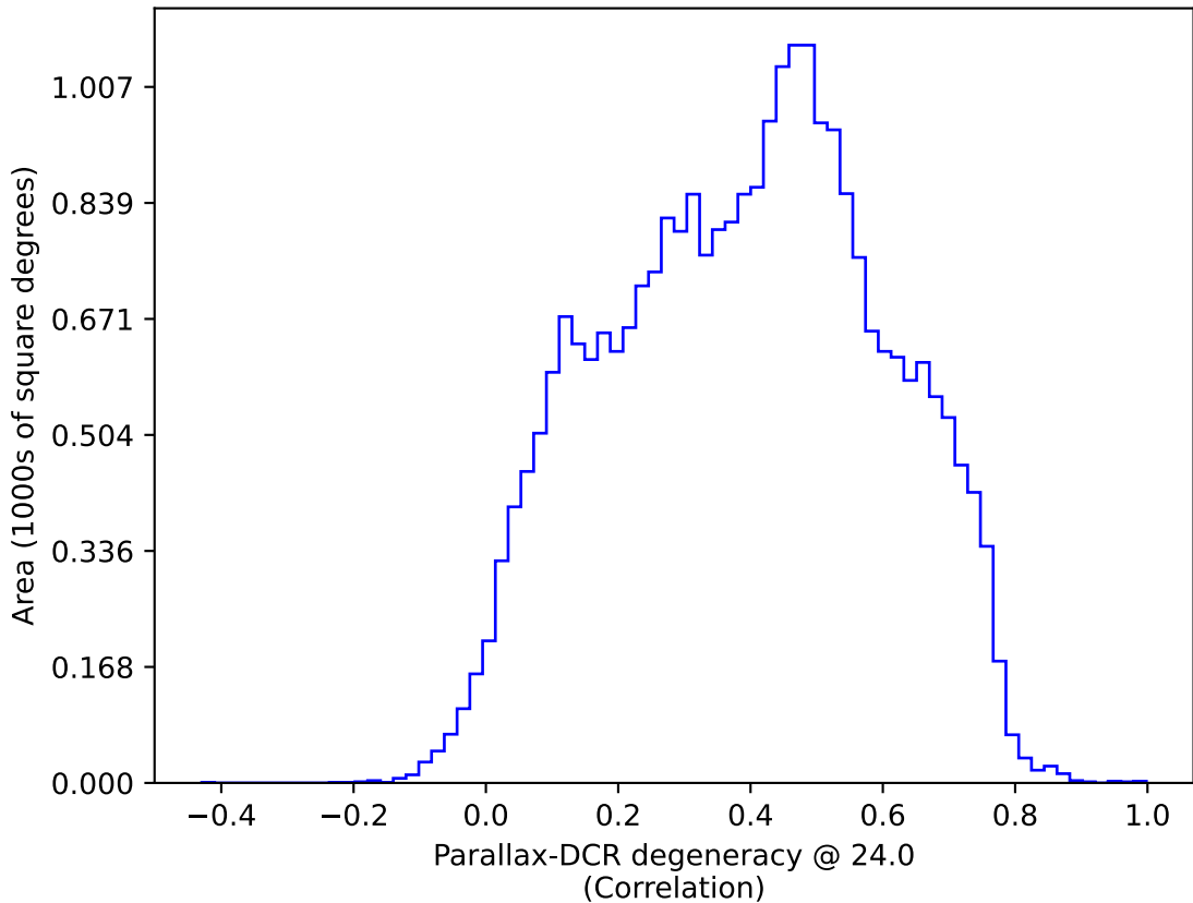
weather_cloudso16v3.4_10yrs All sky: Parallax-DCR degeneracy @ 24.0
