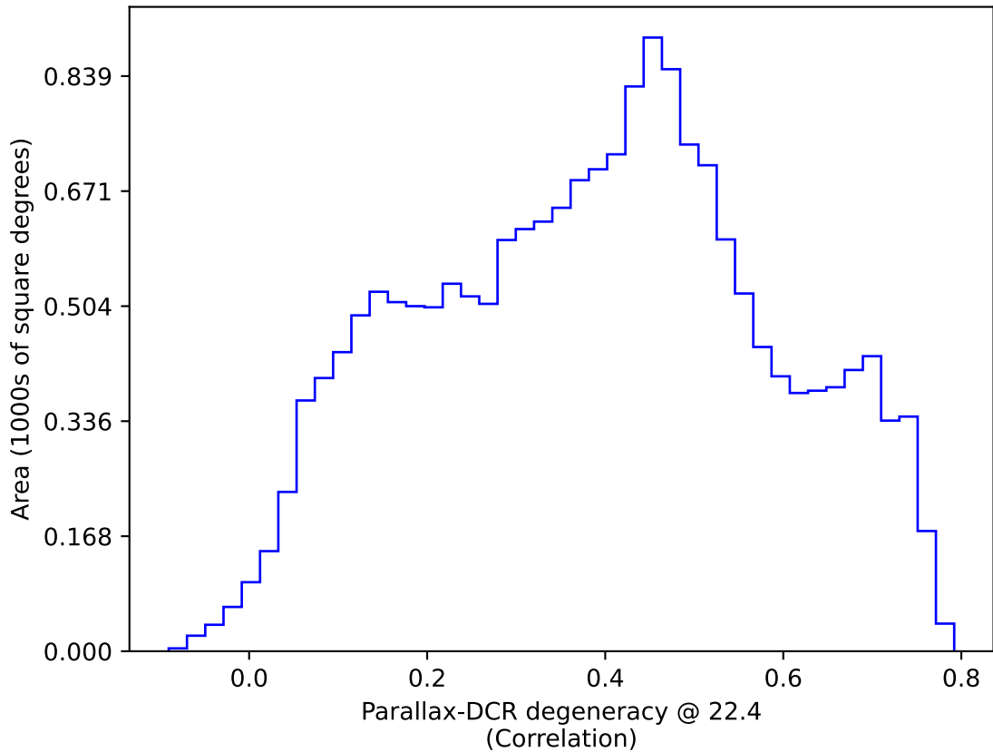
weather_cloudso16v3.4_10yrs WFD: Parallax-DCR degeneracy @ 22.4
