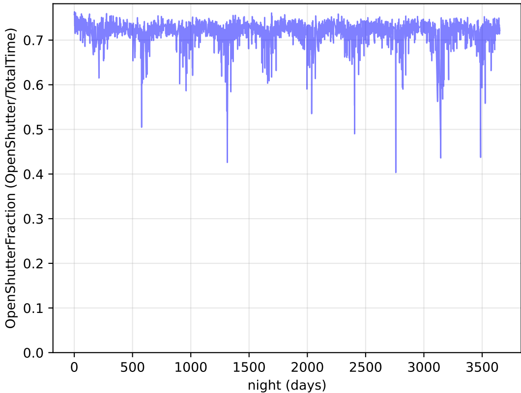
weather_cloudso16v3.4_10yrs Per night: OpenShutterFraction
