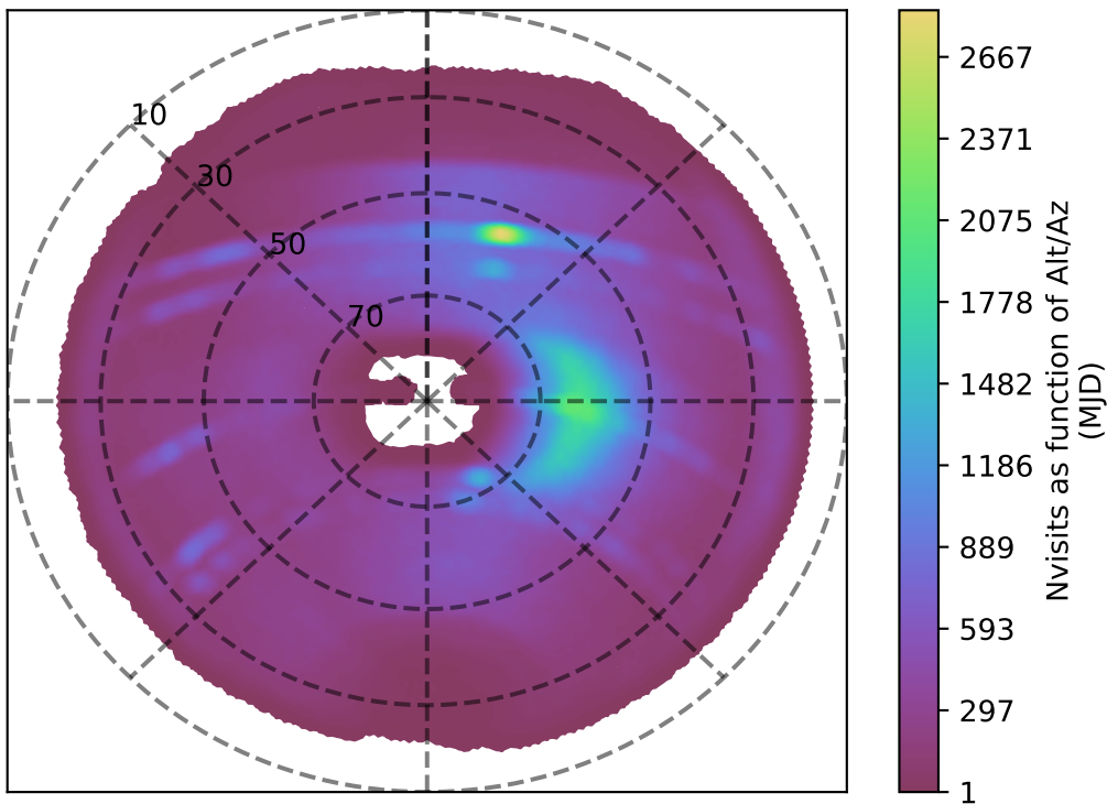
weather_cloudso16v3.4_10yrs z band: Nvisits as function of Alt/Az
