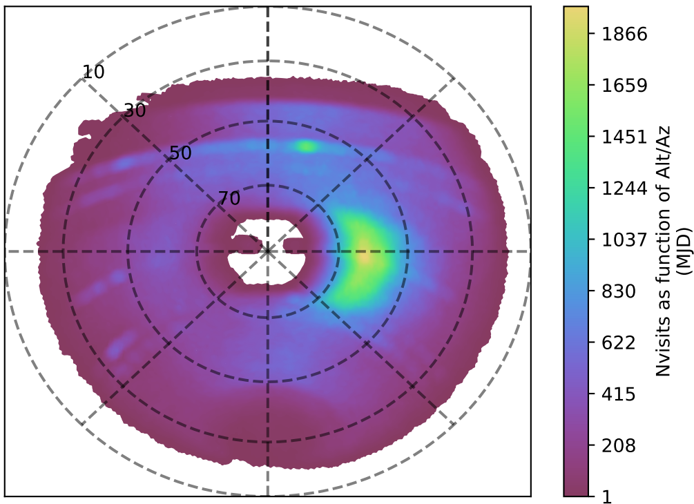
weather_cloudso16v3.4_10yrs y band: Nvisits as function of Alt/Az
