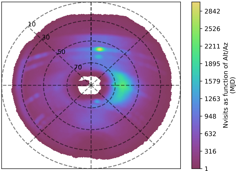
weather_cloudso16v3.4_10yrs r band: Nvisits as function of Alt/Az
