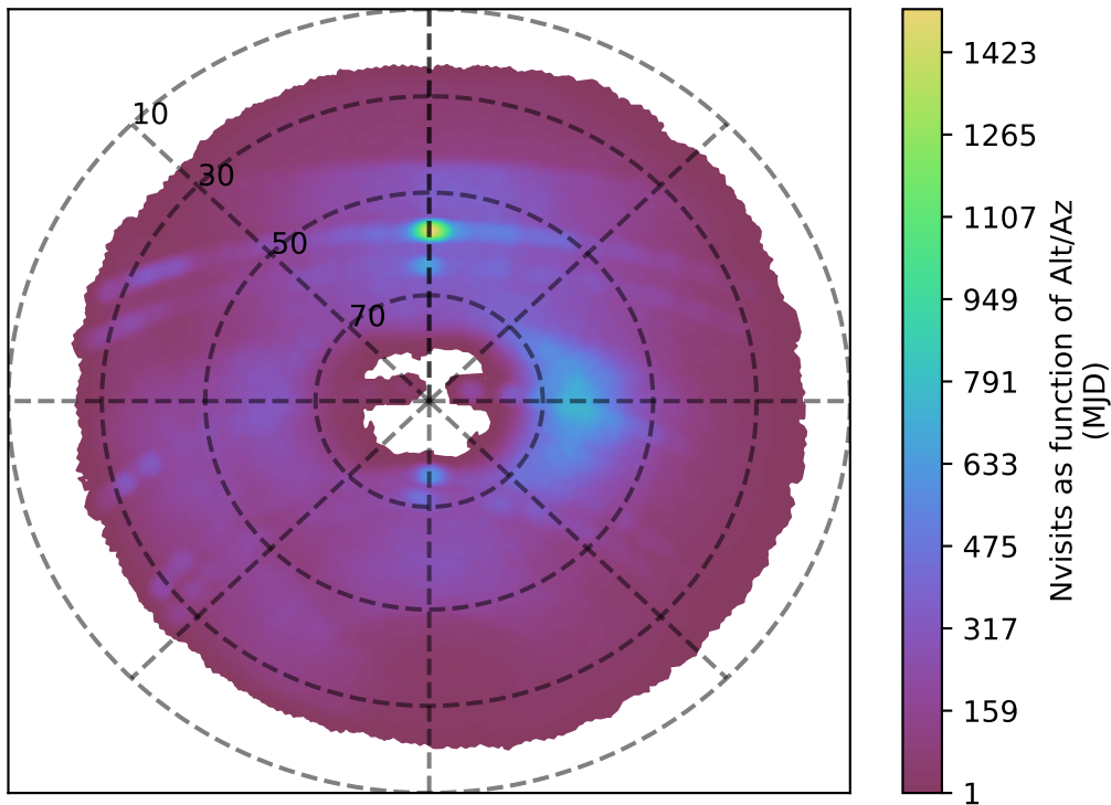
weather_cloudso16v3.4_10yrs g band: Nvisits as function of Alt/Az
