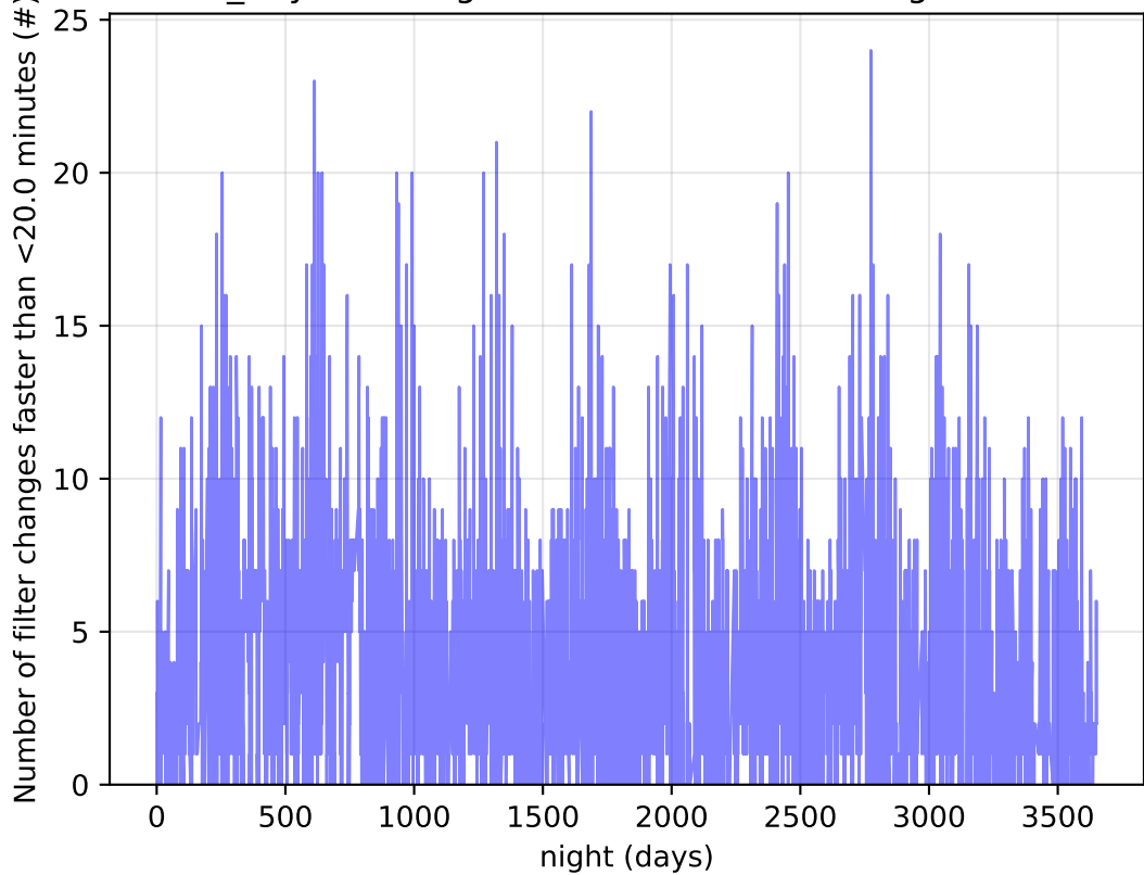
weather_cloudso16v3.4_10yrs Per Night: Number of filter changes faster than <20.0 minutes
