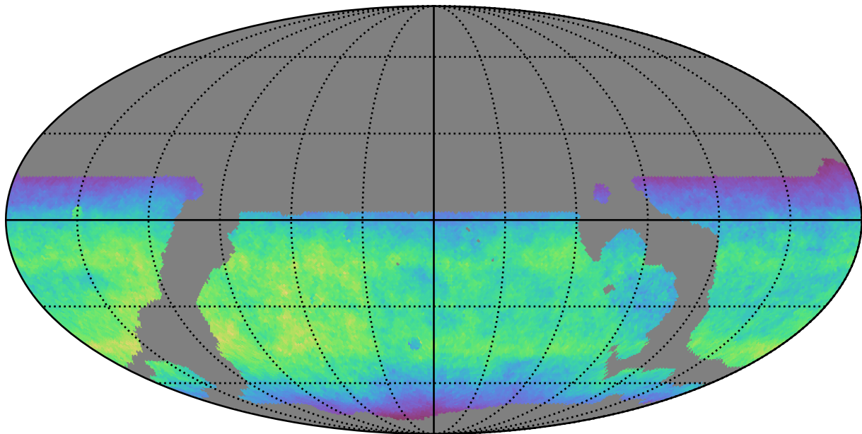
weather_cloudso16v3.4_10yrs WFD y band: Normalized Teff
