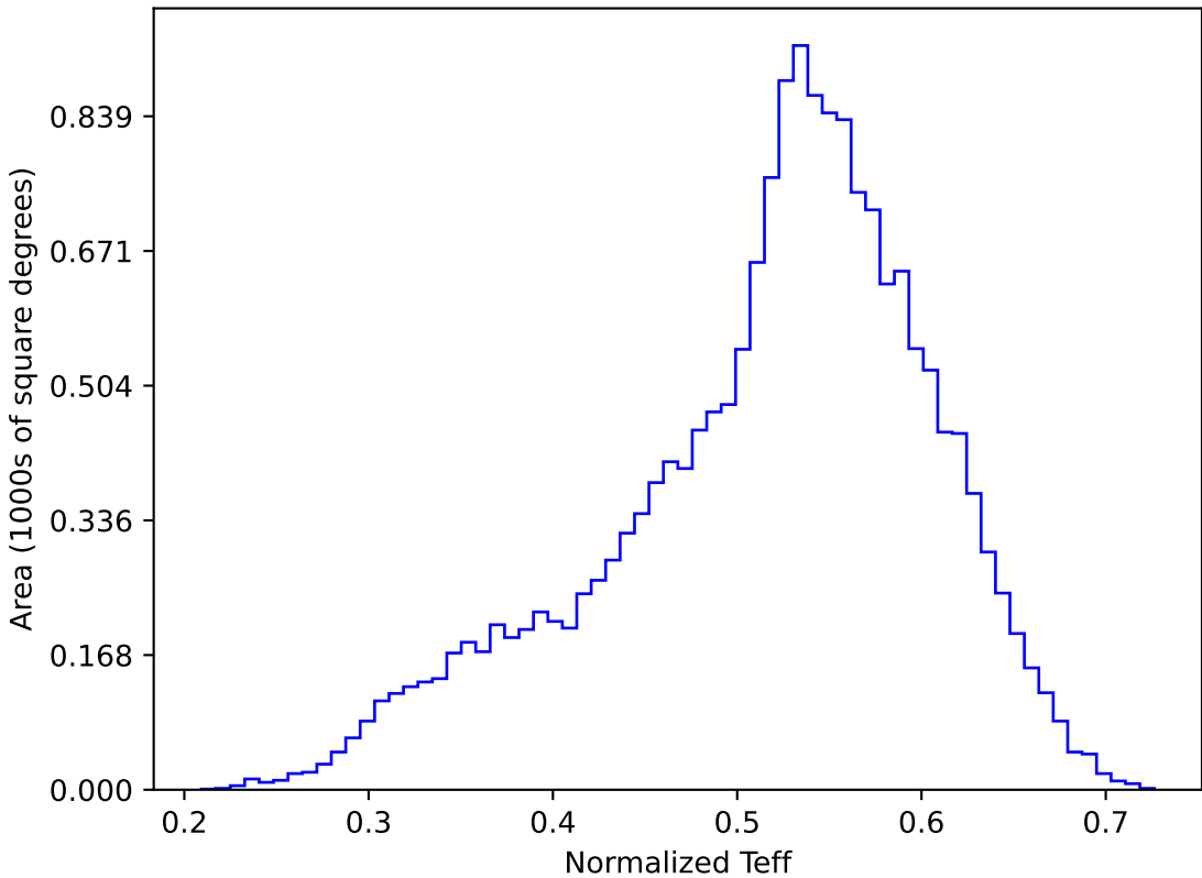
weather_cloudso16v3.4_10yrs WFD y band: Normalized Teff
