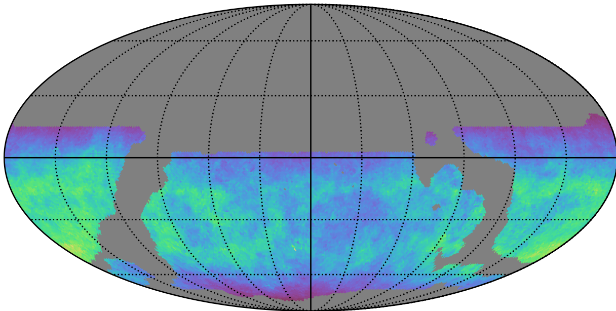
weather_cloudso16v3.4_10yrs WFD u band: Normalized Teff
