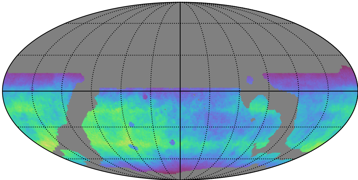
weather_cloudso16v3.4_10yrs WFD r band: Normalized Teff
