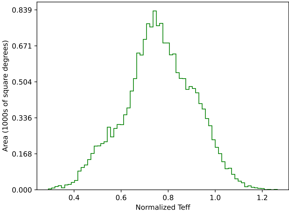
weather_cloudso16v3.4_10yrs WFD g band: Normalized Teff
