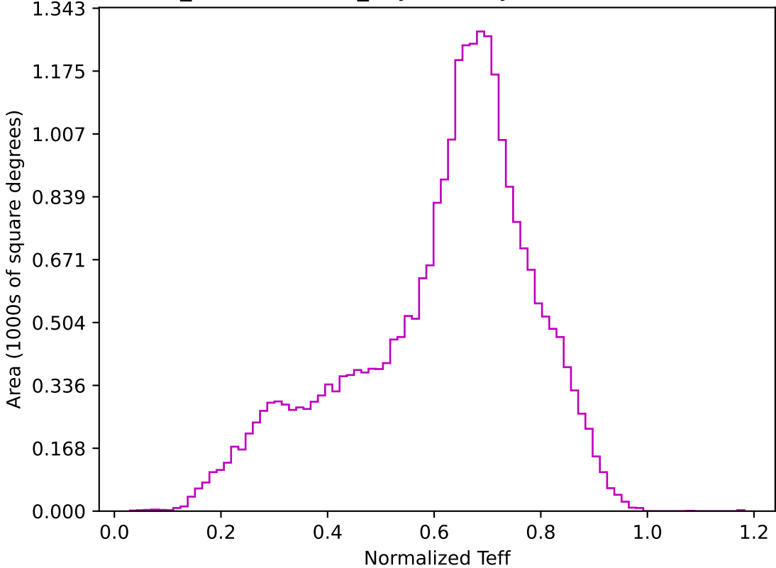
weather_cloudso16v3.4_10yrs All sky z band: Normalized Teff
