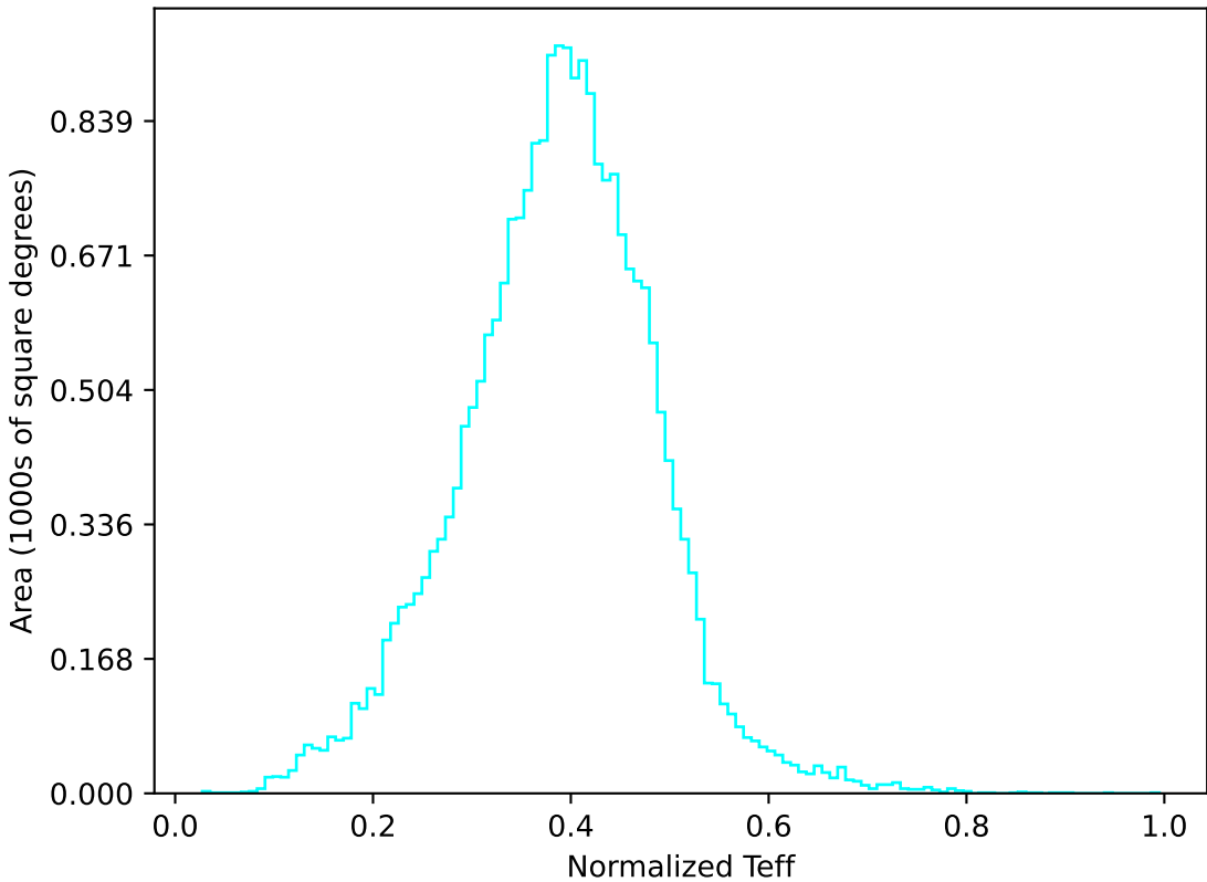
weather_cloudso16v3.4_10yrs All sky u band: Normalized Teff
