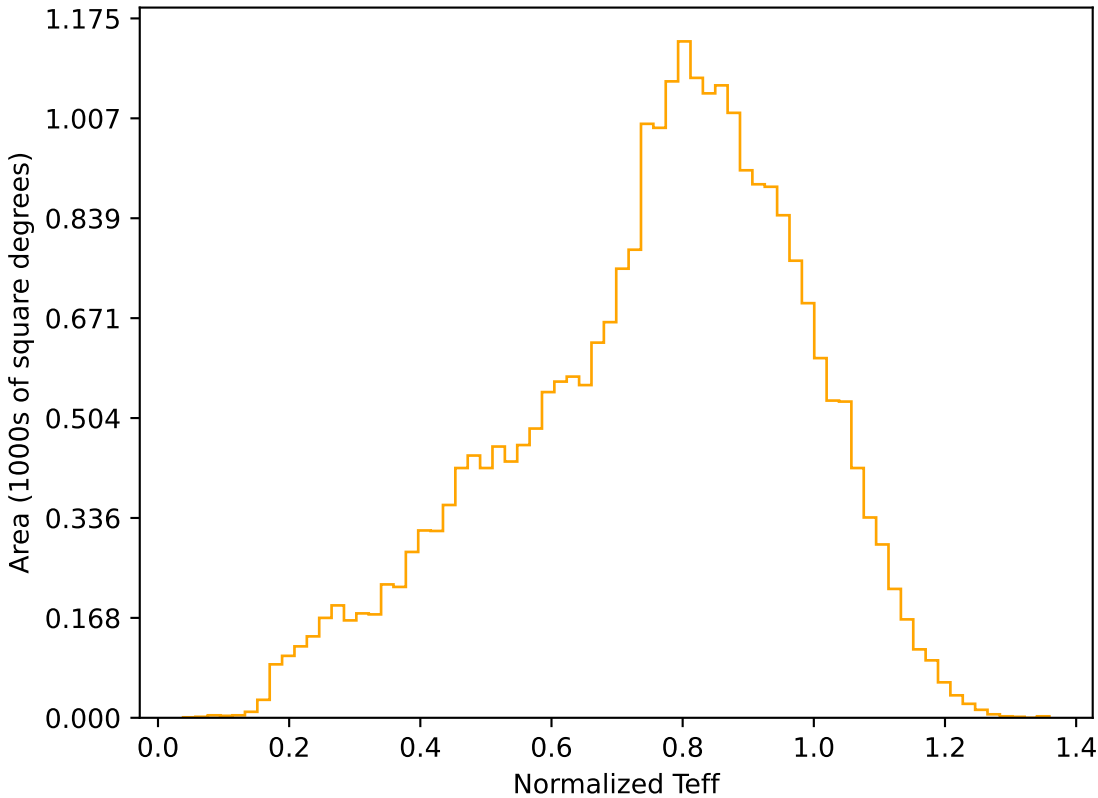
weather_cloudso16v3.4_10yrs All sky r band: Normalized Teff
