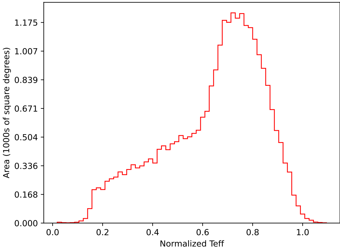
weather_cloudso16v3.4_10yrs All sky i band: Normalized Teff
