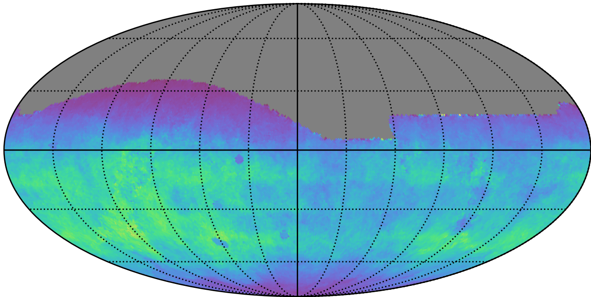
weather_cloudso16v3.4_10yrs All sky g band: Normalized Teff
