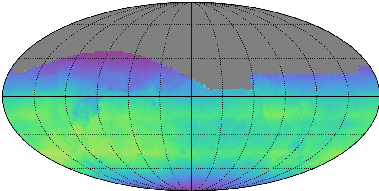
weather_cloudso16v3.4_10yrs All sky all bands: Normalized Teff
