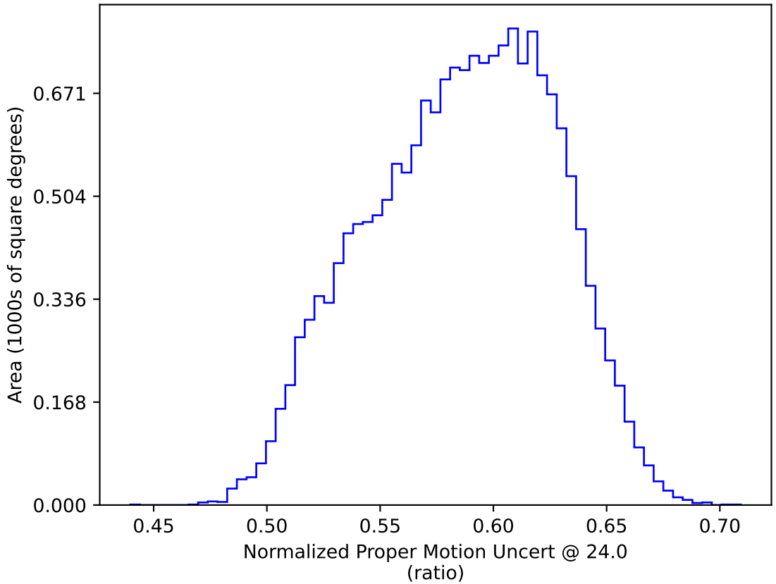
weather_cloudso16v3.4_10yrs WFD: Normalized Proper Motion Uncert @ 24.0
