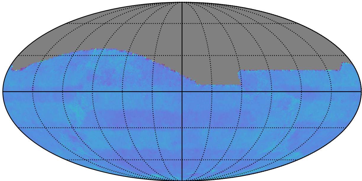
weather_cloudso16v3.4_10yrs All sky: Normalized Proper Motion Uncert @ 24.0
