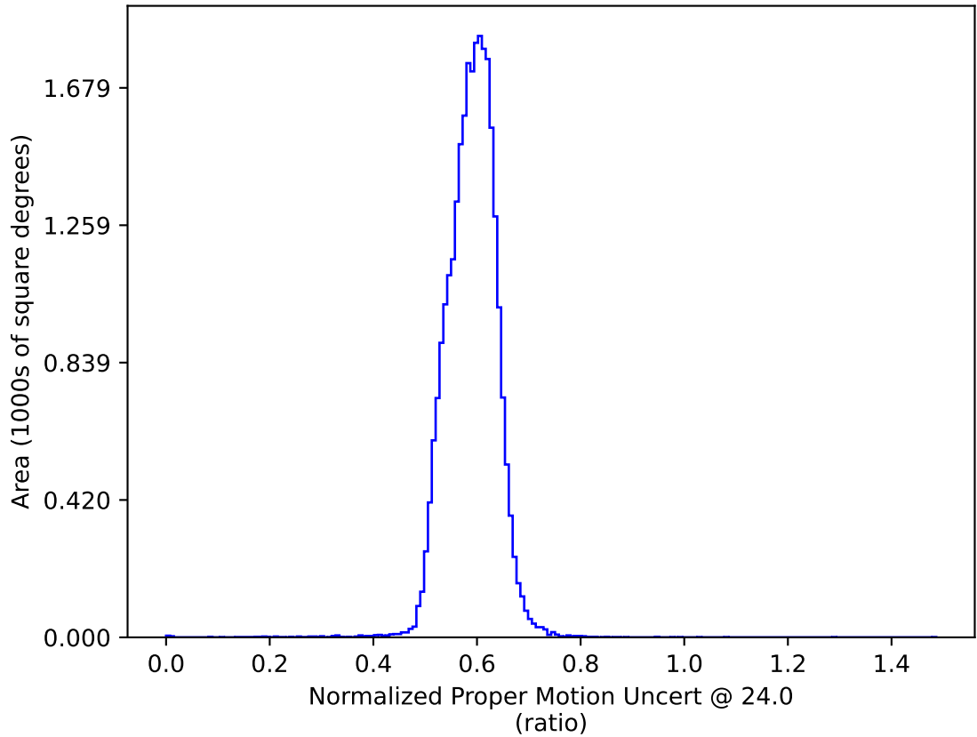
weather_cloudso16v3.4_10yrs All sky: Normalized Proper Motion Uncert @ 24.0
