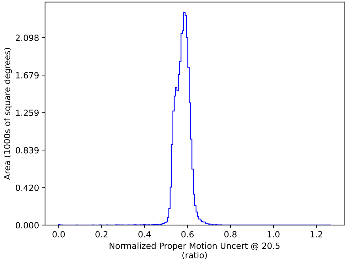
weather_cloudso16v3.4_10yrs All sky: Normalized Proper Motion Uncert @ 20.5
