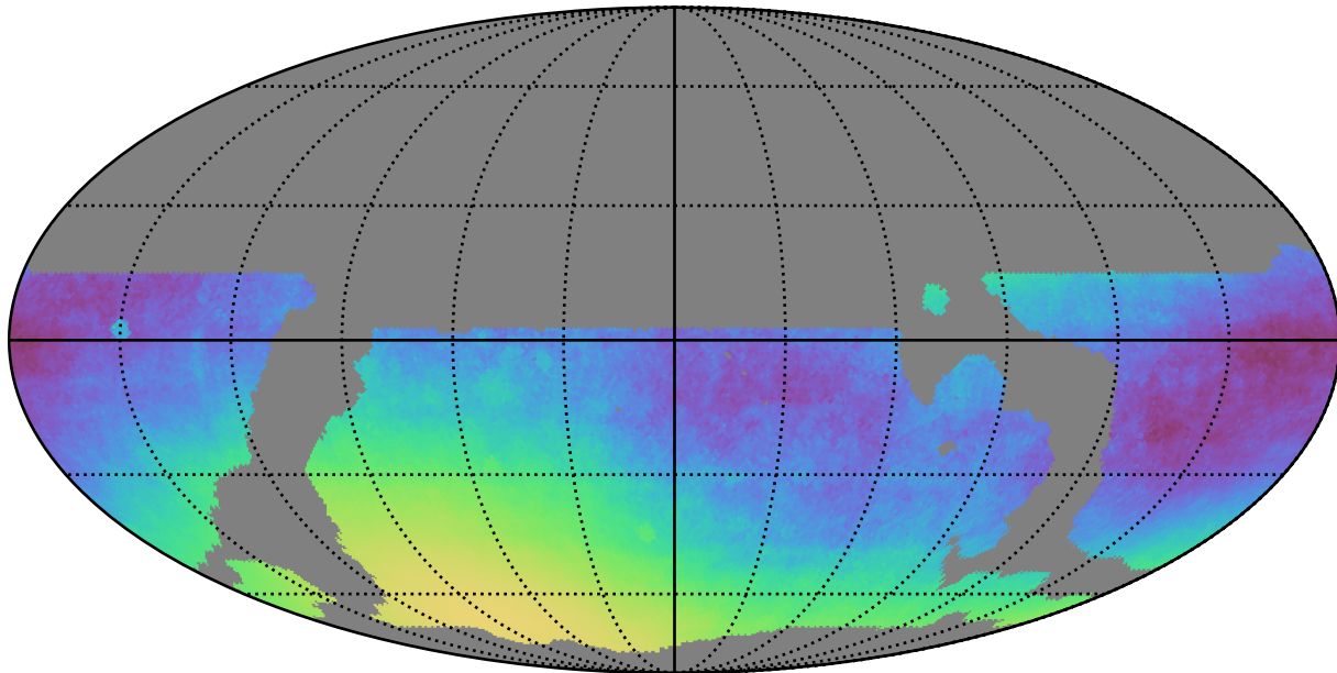
weather_cloudso16v3.4_10yrs WFD: Normalized Parallax Uncert @ 24.0
