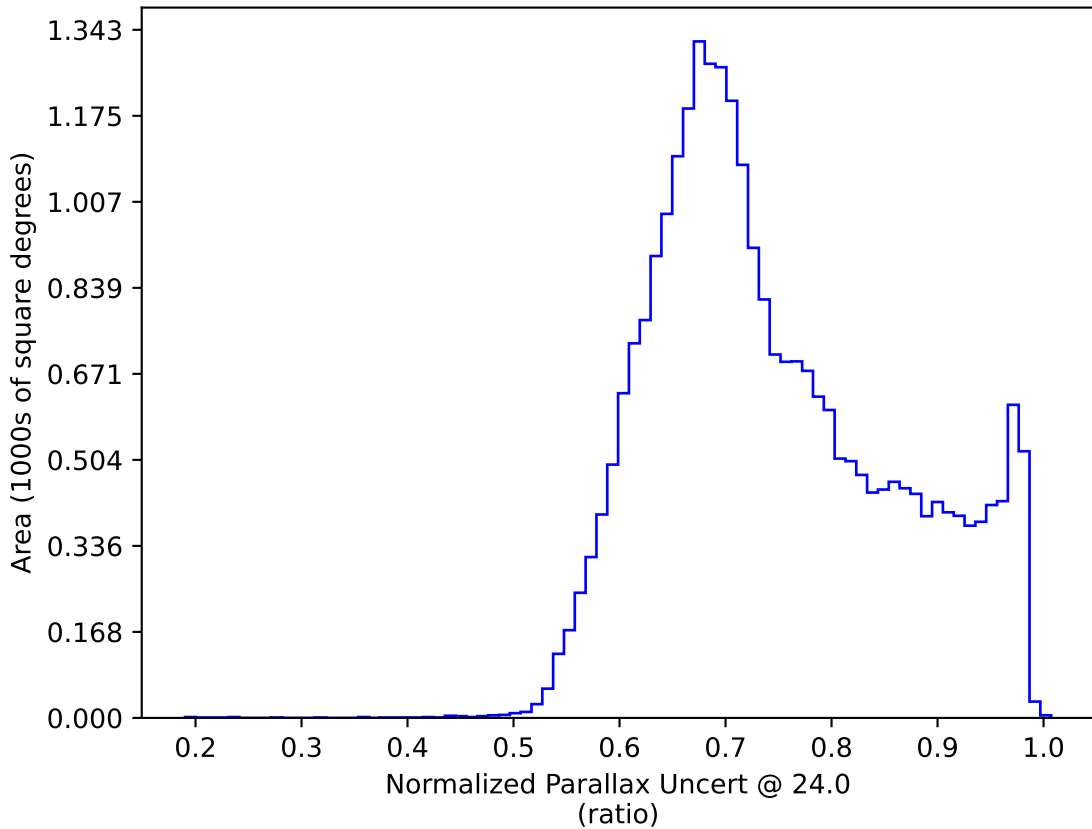
weather_cloudso16v3.4_10yrs All sky: Normalized Parallax Uncert @ 24.0
