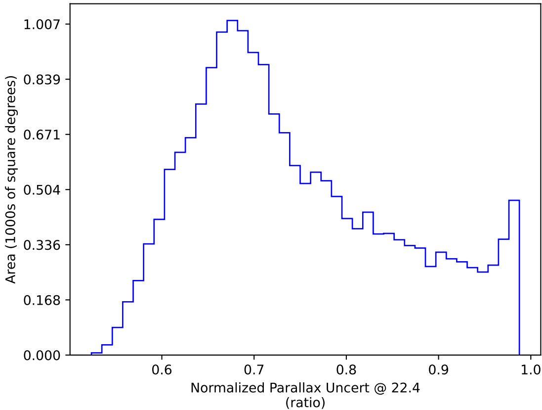
weather_cloudso16v3.4_10yrs WFD: Normalized Parallax Uncert @ 22.4
