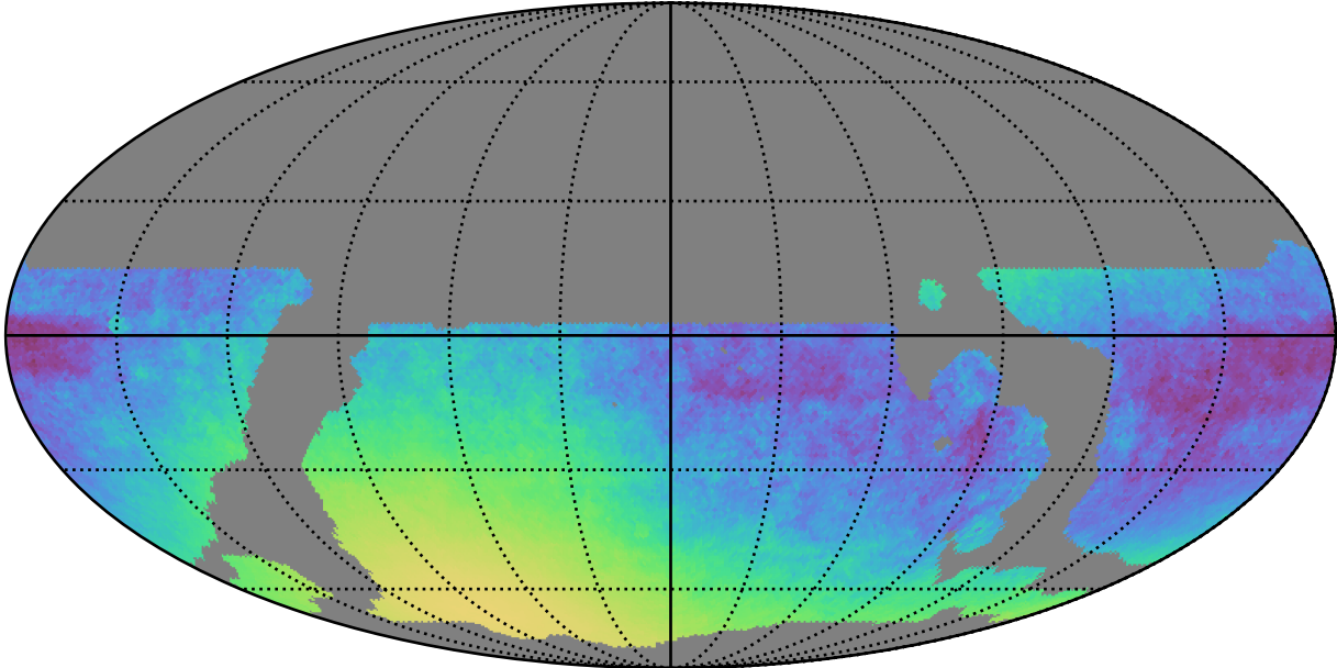
weather_cloudso16v3.4_10yrs WFD y band only: Normalized Parallax Uncert @ 21.3
