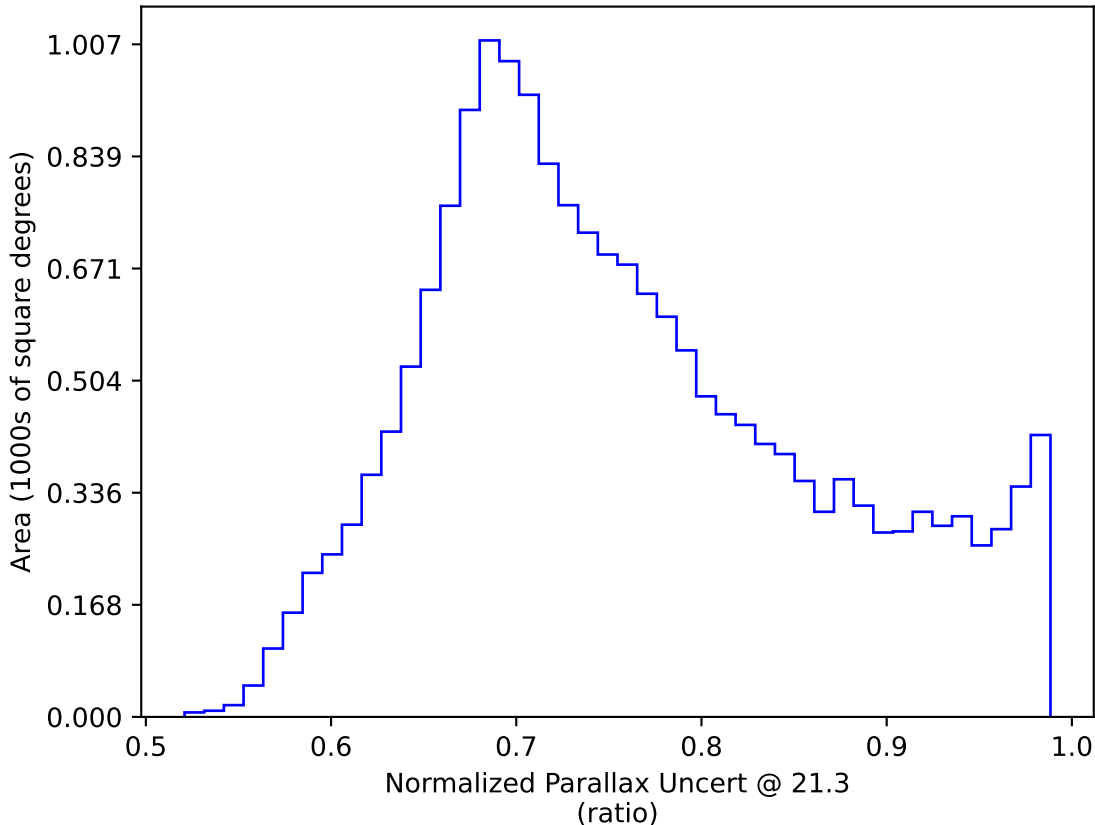
weather_cloudso16v3.4_10yrs WFD y band only: Normalized Parallax Uncert @ 21.3
