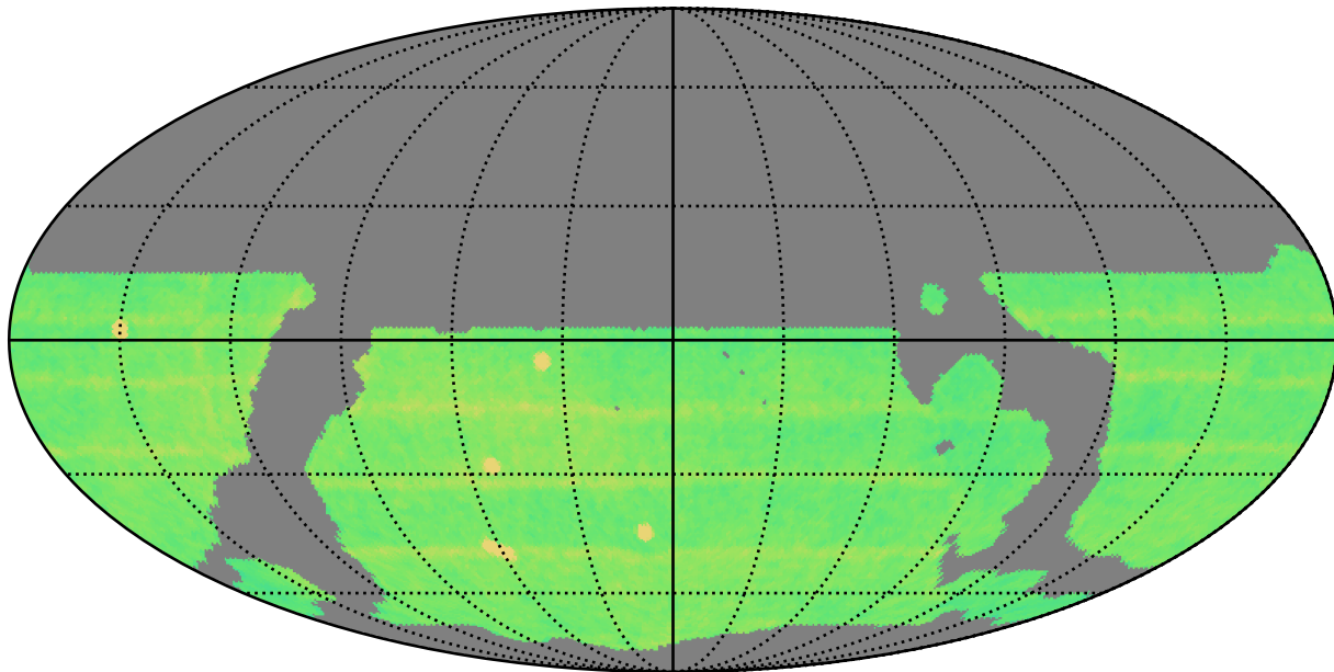
weather_cloudso16v3.4_10yrs WFD all bands: N Unique Nights
