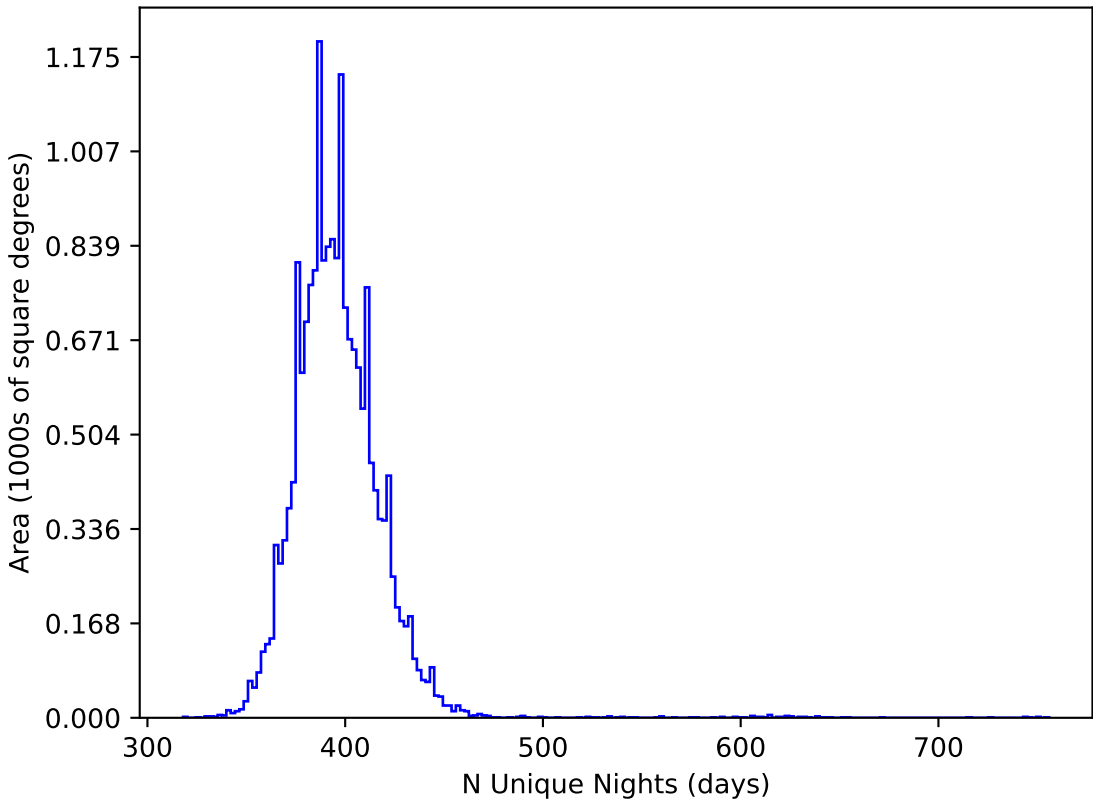
weather_cloudso16v3.4_10yrs WFD all bands: N Unique Nights
