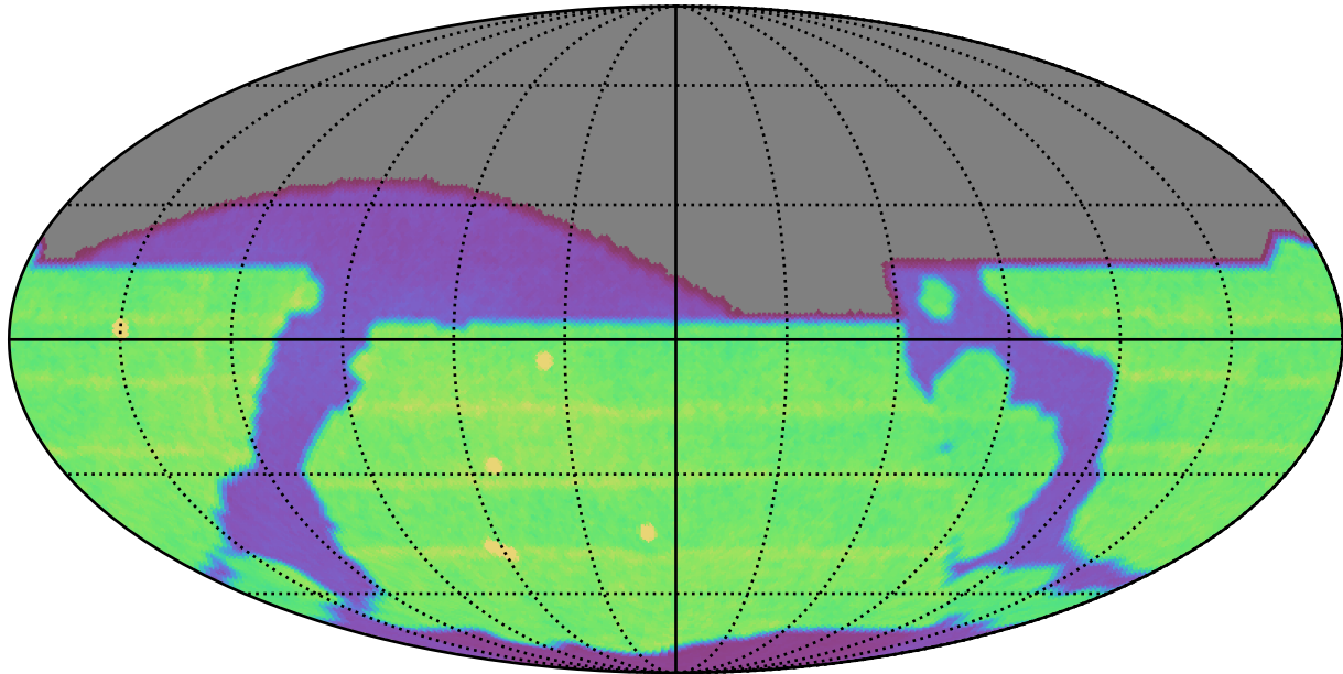
weather_cloudso16v3.4_10yrs All sky all bands: N Unique Nights
