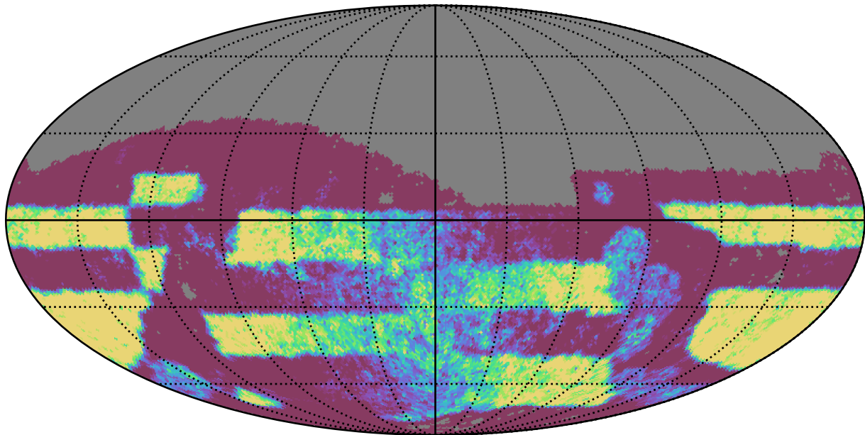
weather_cloudso16v3.4_10yrs Yr 3-4 z band: NVisits
